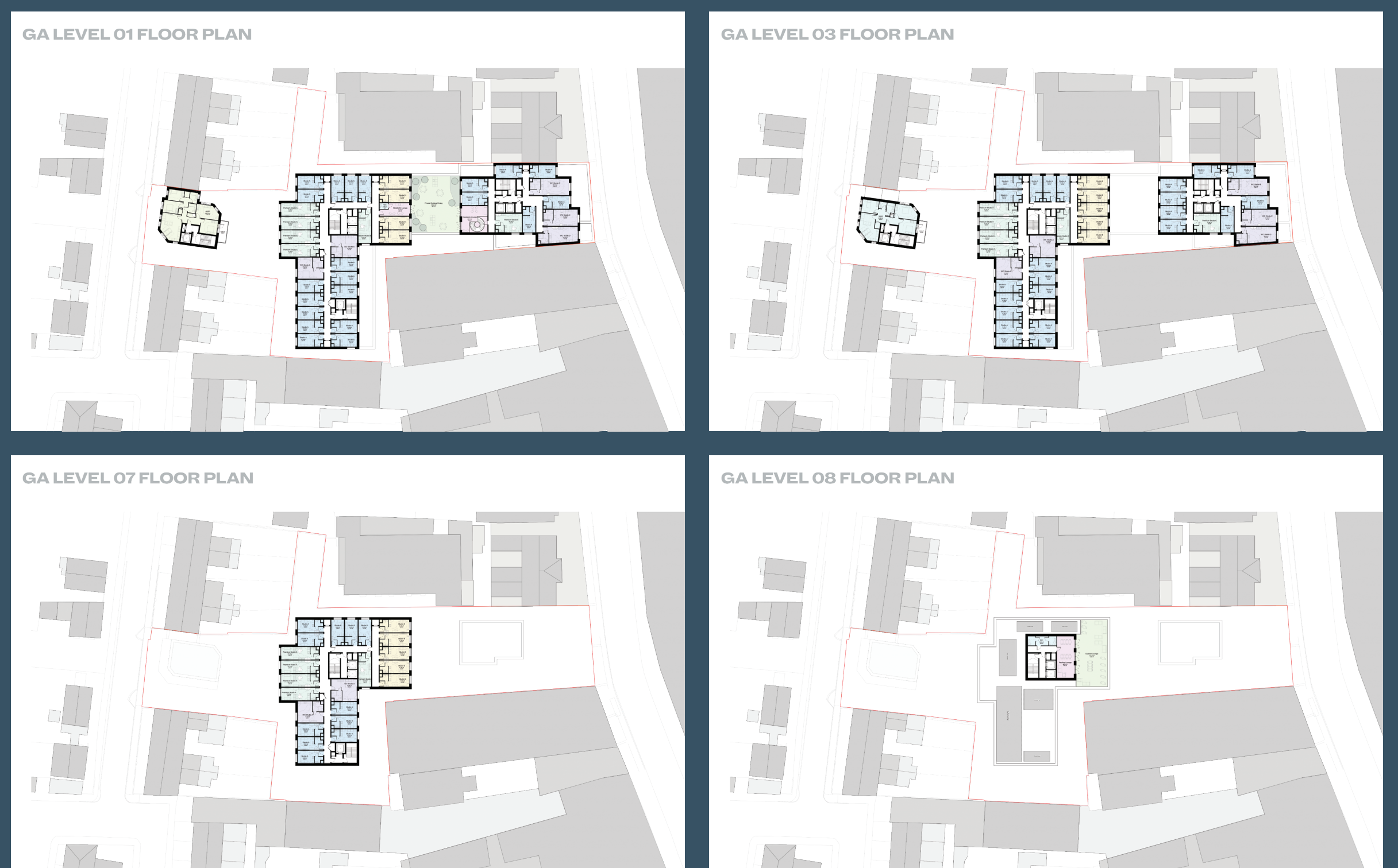
Indicative floor plans illustrating the different heights of the proposed buildings on the site
